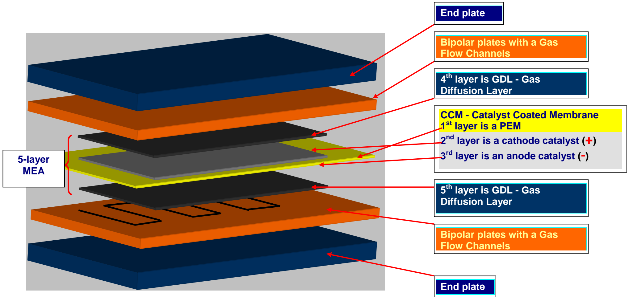
Fig.1 Extended view of benchmark's PEM Fuel Cell (with 5-layer MEA)
